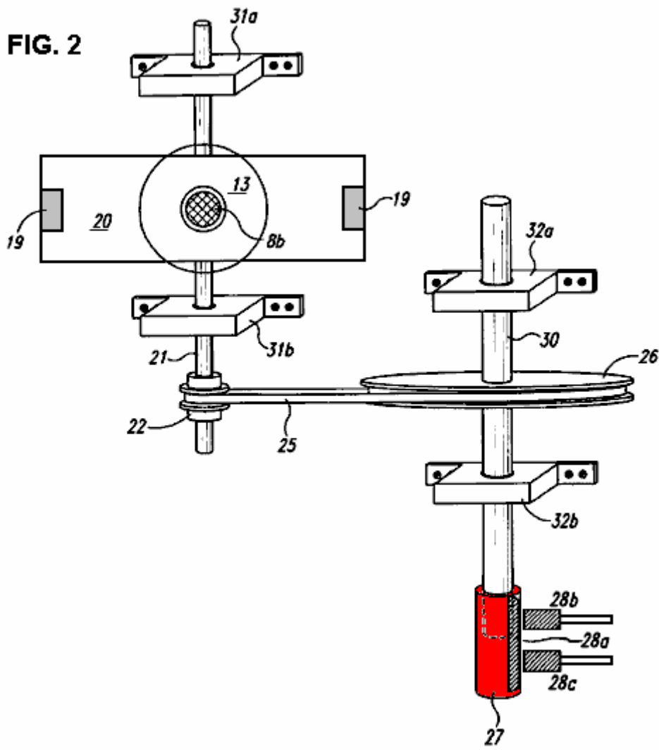
Fig.2 is a perspective top view of a monopole back EMF motor with a single stator and a single rotor.
